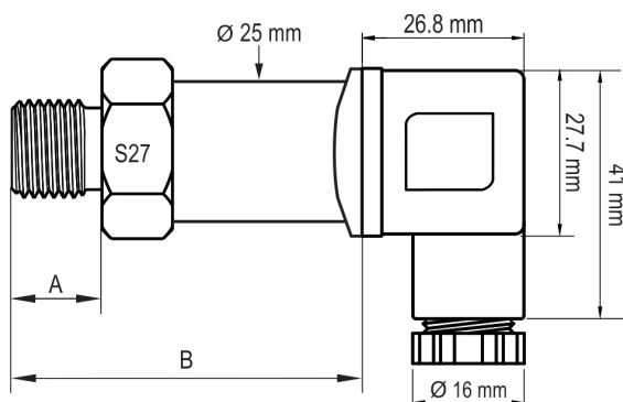
Fig. 3 – Transmitter dimensions
